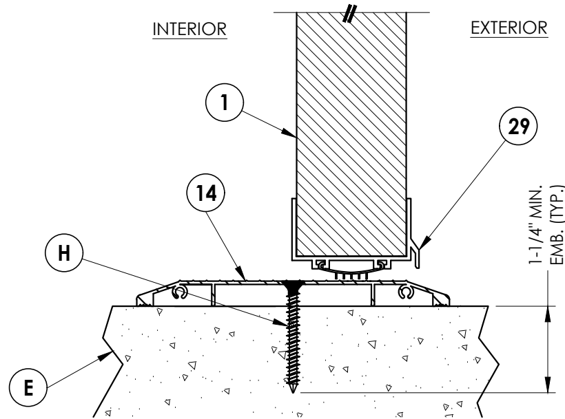
5 4 VERTICAL CROSS SECTION
