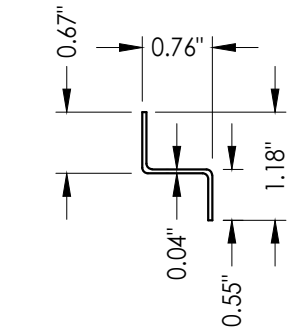
12 MULLION Z BRACKET
